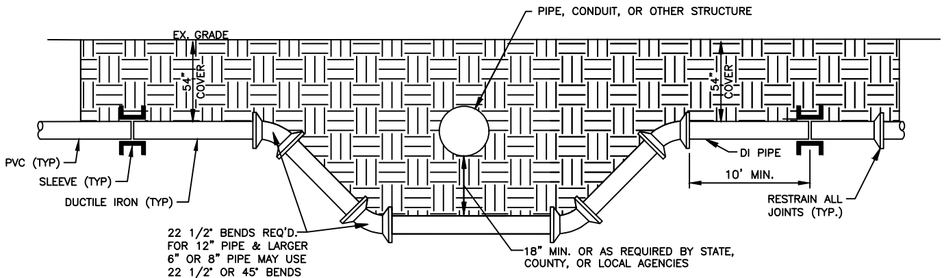
PVC PIPE WITH DUCTILE IRON PIPE
