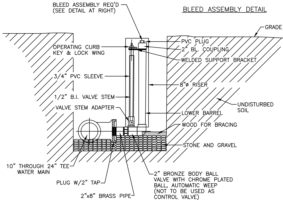
SECTION
