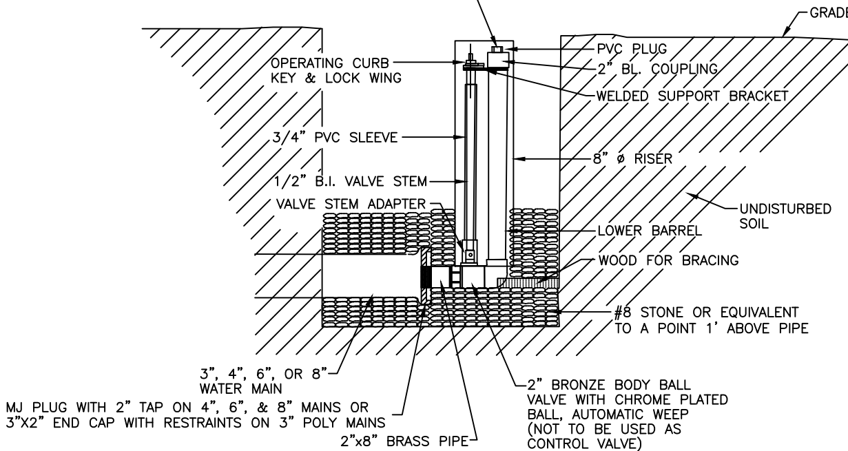
SECTION
