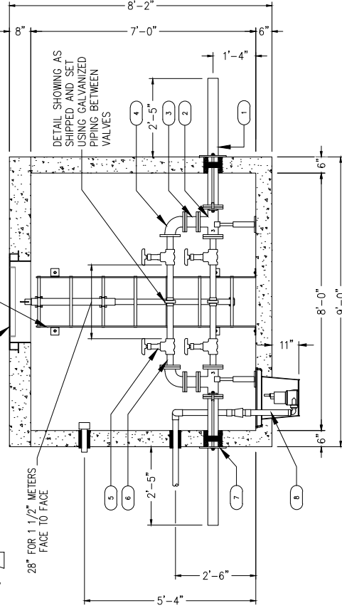
2 SECTION VIEW 1" = 3'-0"
