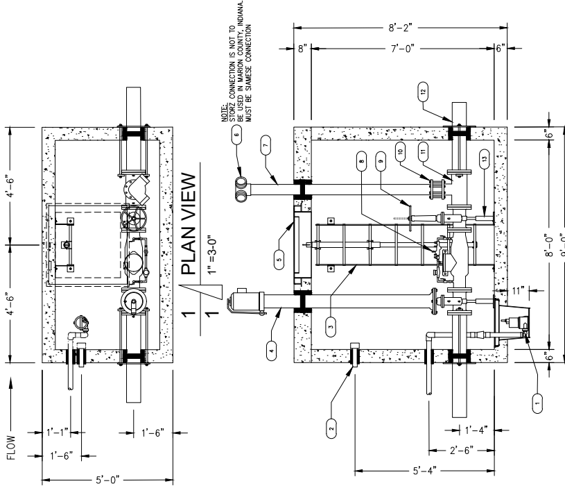
1 PLAN VIEW 1" = 3'-0"
