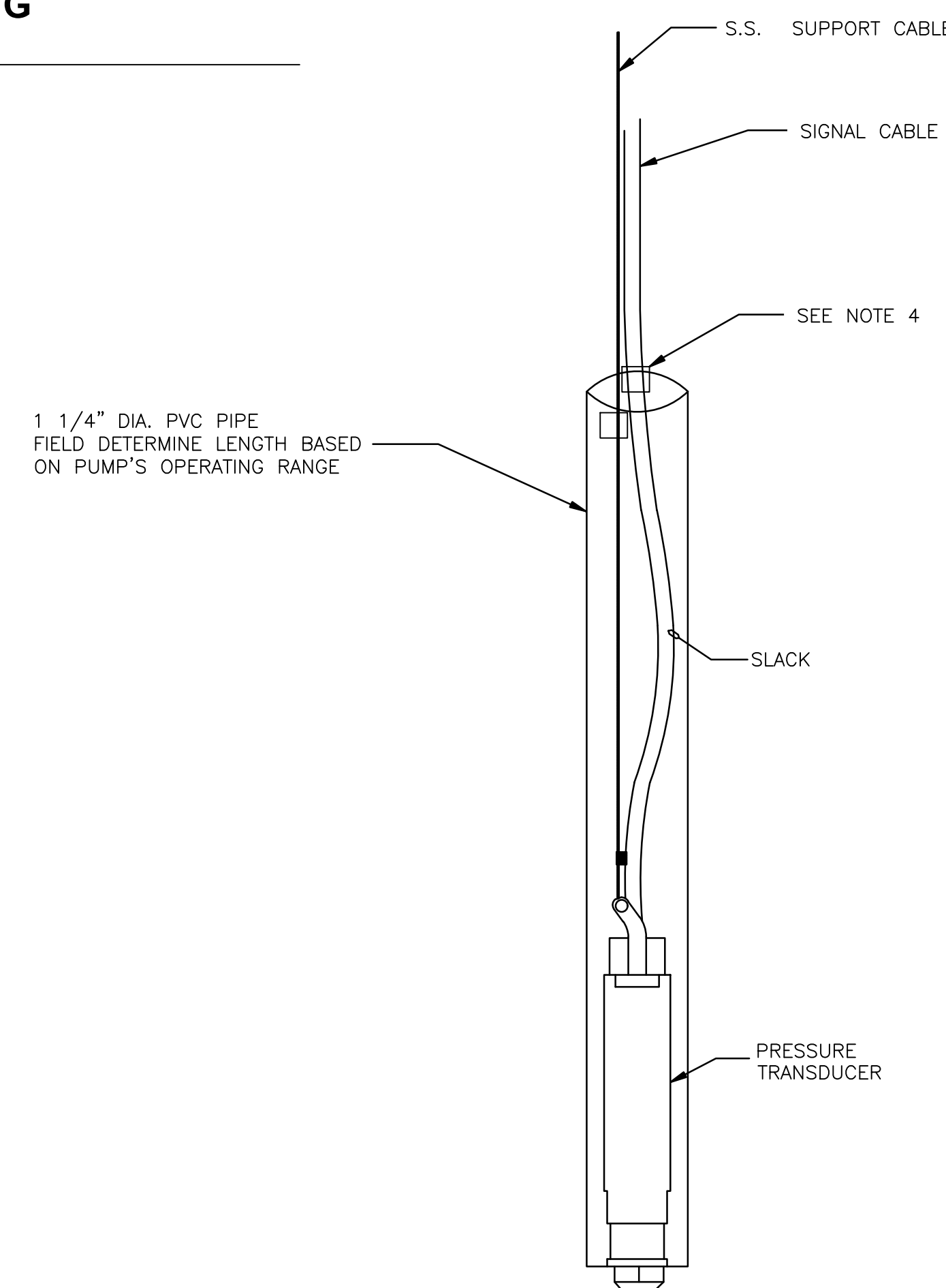
PRESSURE TRANSDUCER DETAIL
