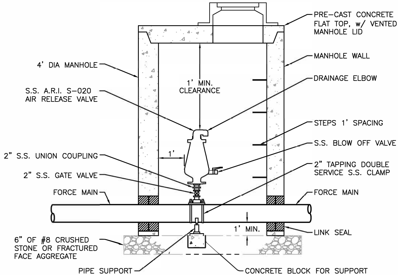
TYPICAL AIR RELEASE VALVE DETAIL
