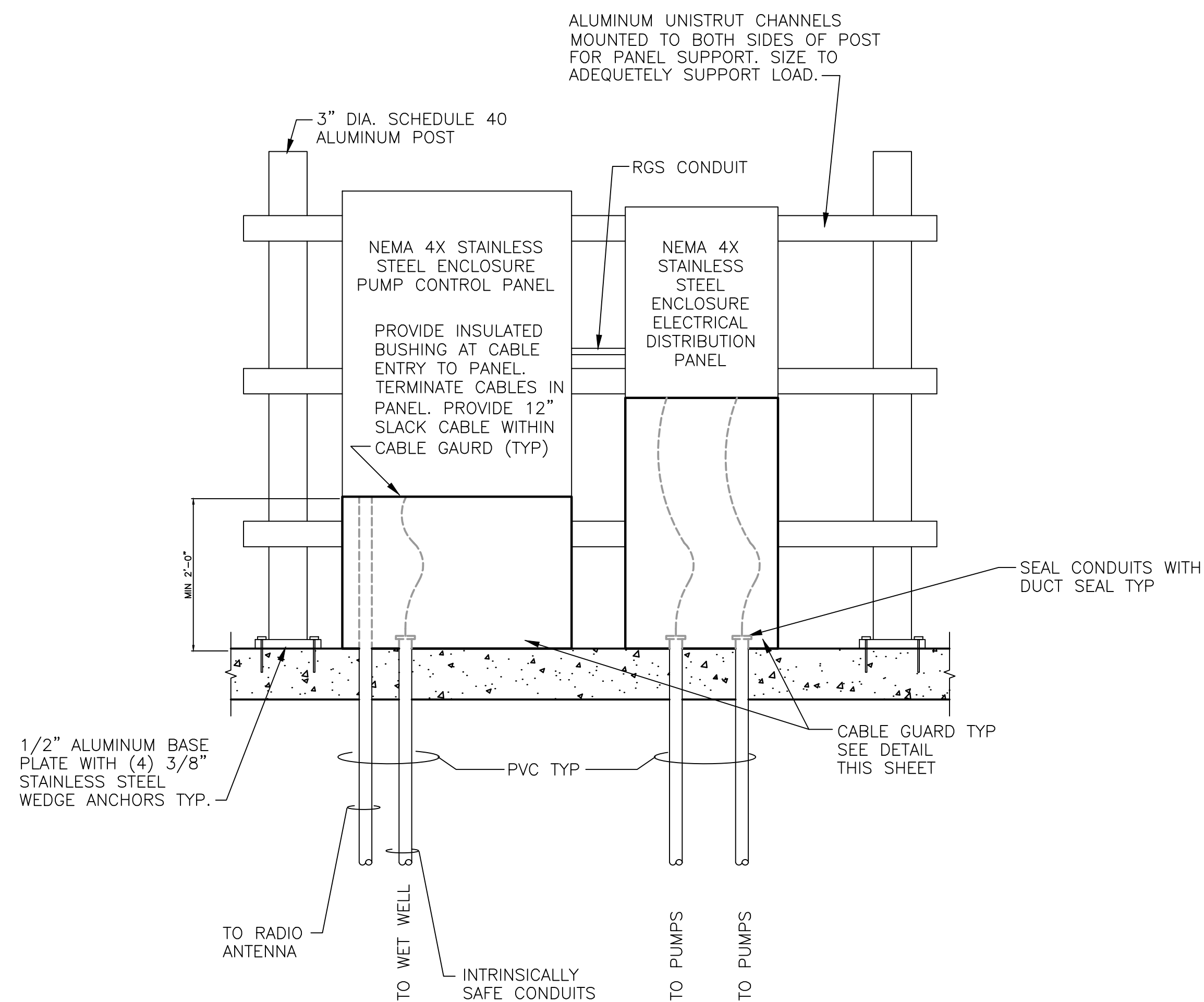
EQUIPMENT MOUNTING DETAIL (FRONT)
