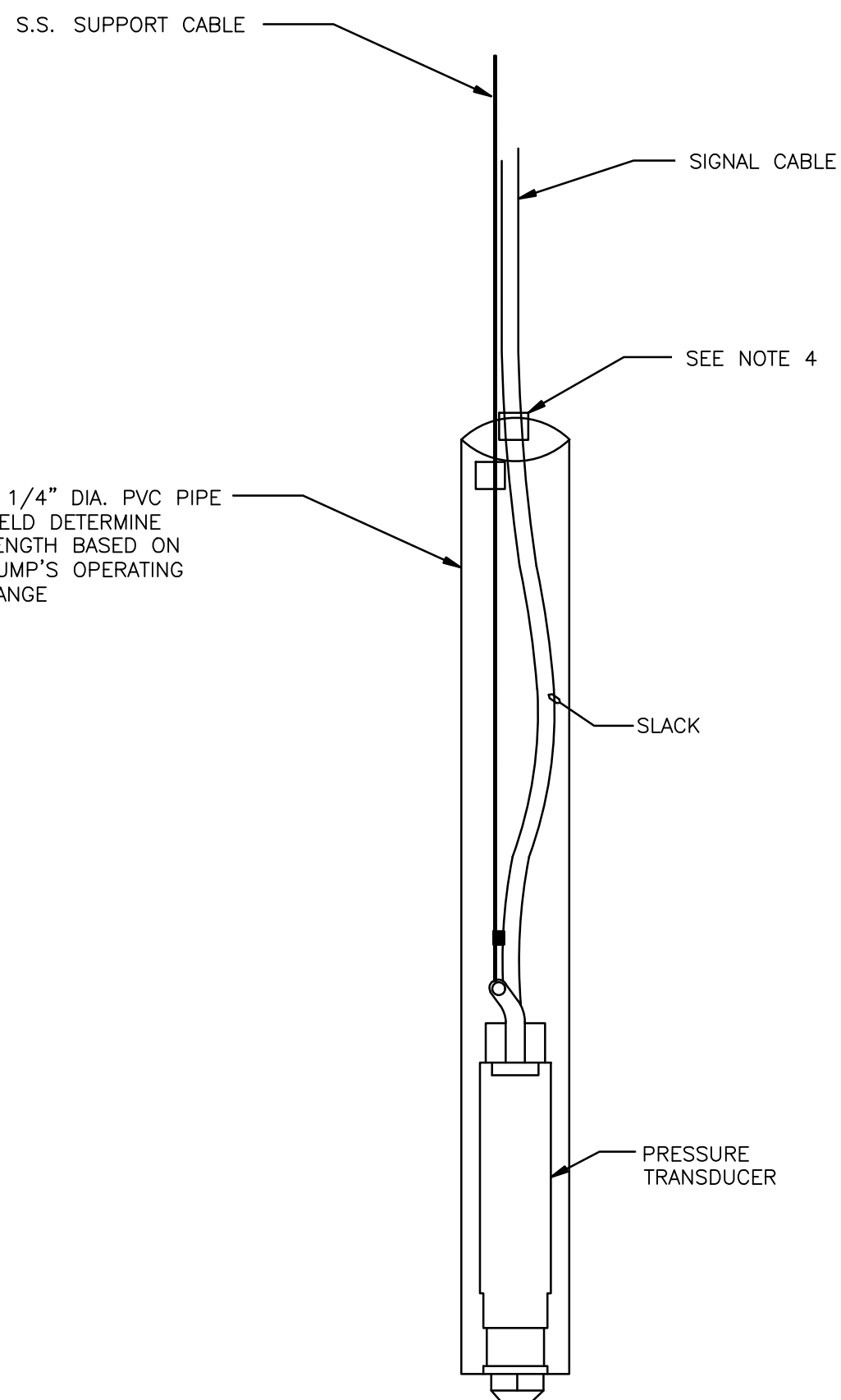
PRESSURE TRANSDUCER DETAIL
