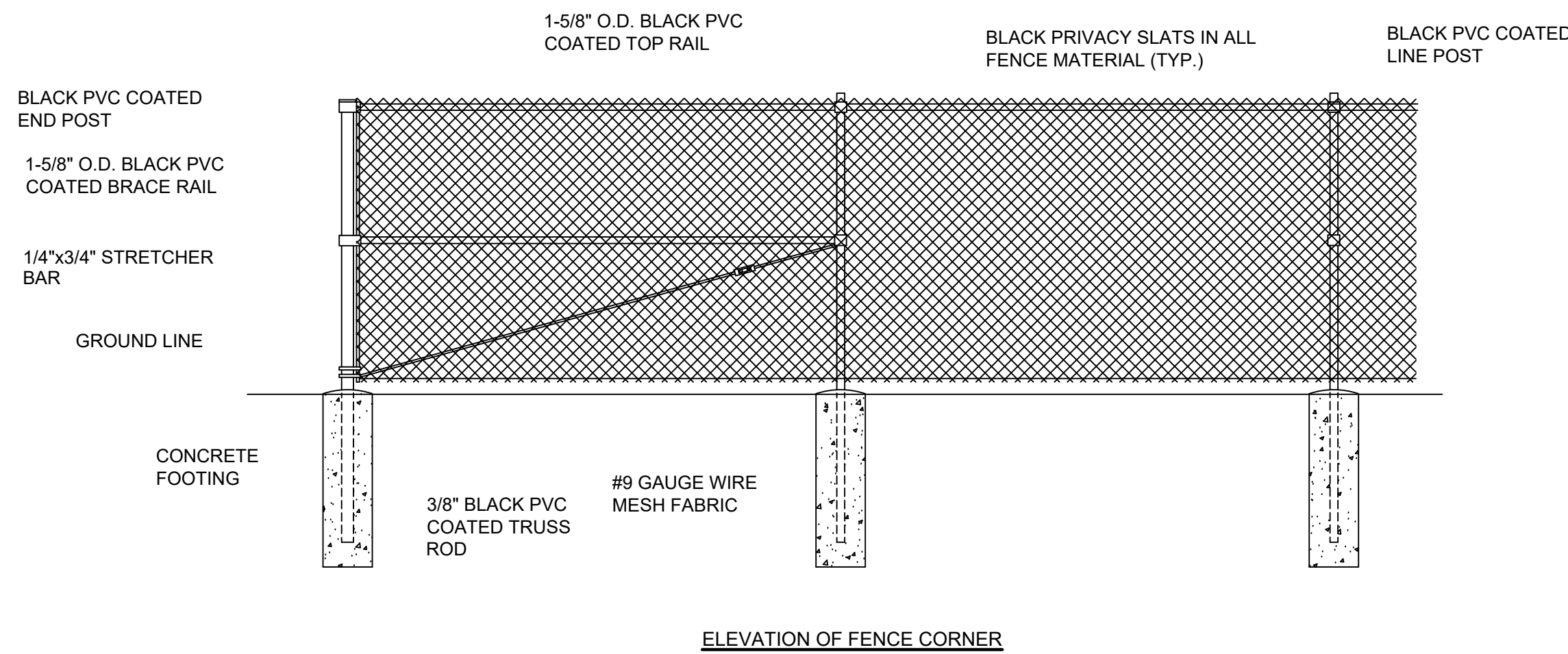
CHAINLINK FENCE DETAIL 13 SCALE: NONE
