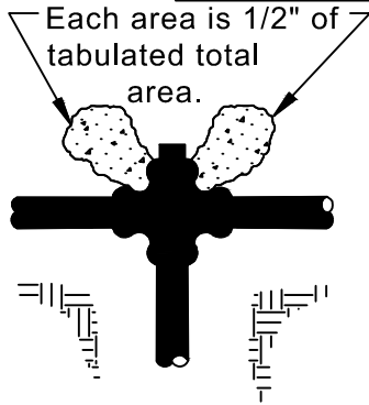
PLUGGED CROSS
