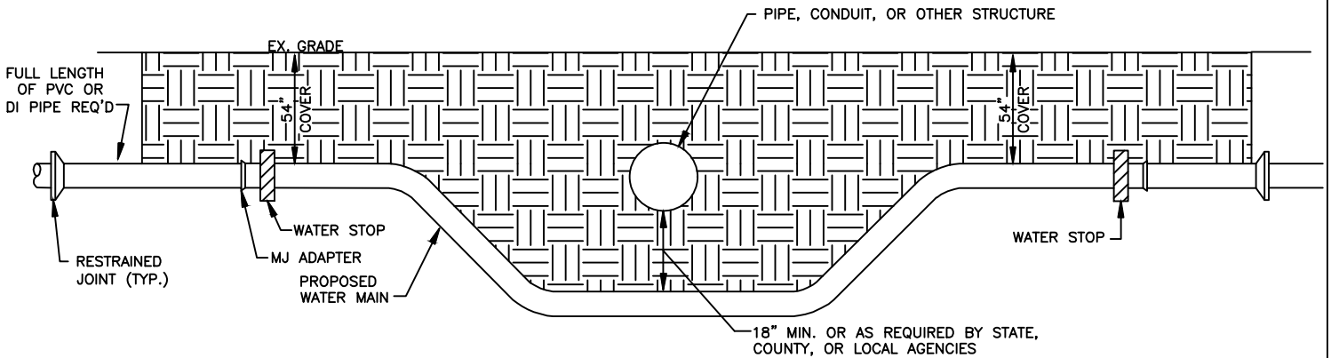
POLYETHYLENE PIPE
