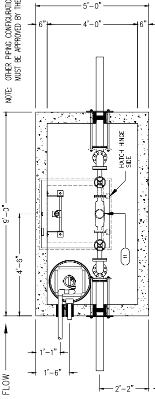
1 PLAN VIEW 1" = 3'-0"
