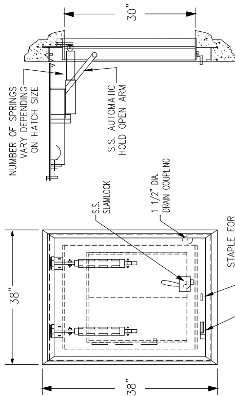
PLAN VIEW 38" x 38" overall hatch size 30" diameter opening
