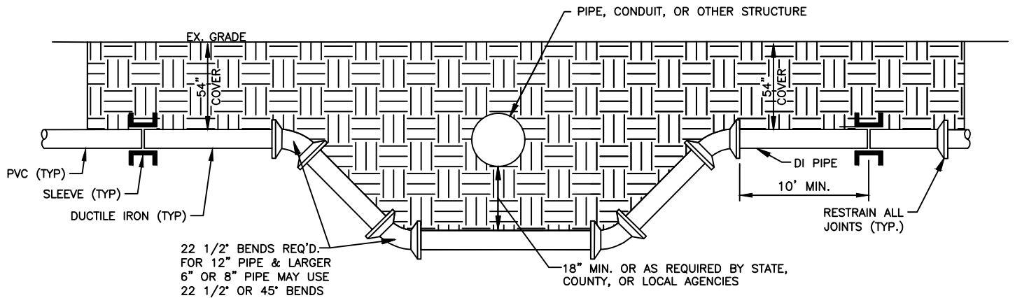
PVC PIPE WITH DUCTILE IRON PIPE
