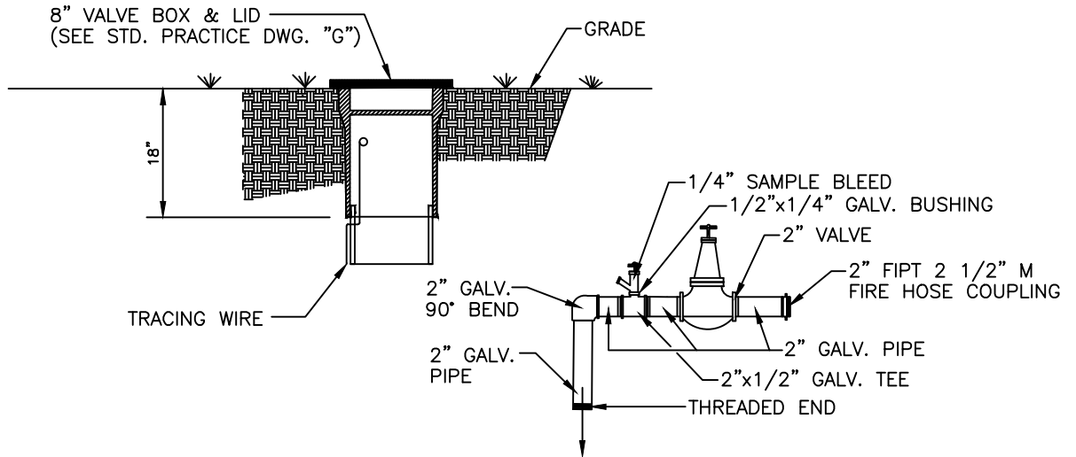
BLEED ASSEMBLY DETAIL
