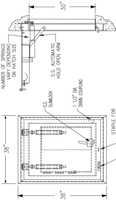
SECTION VIEW SIDE
