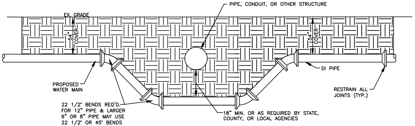
DUCTILE IRON PIPE
