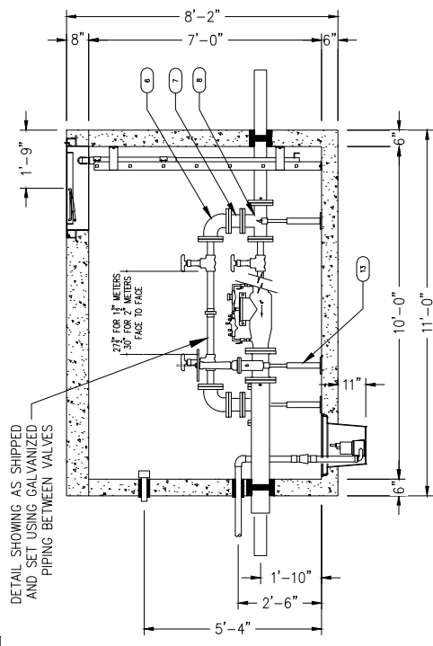
1 PLAN VIEW 1" = 3'-0"
