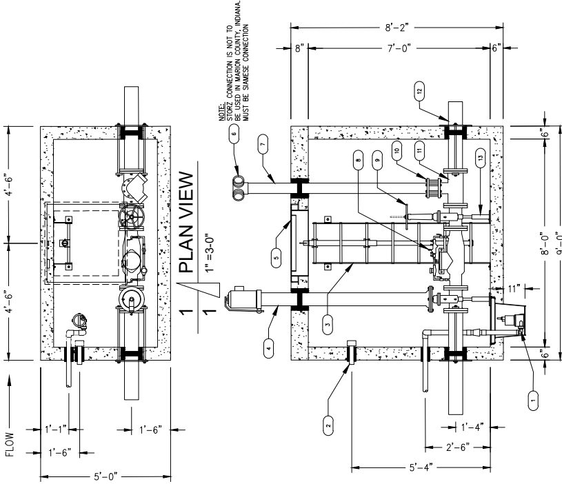
1 PLAN VIEW 1" = 3'-0" 2 SECTION VIEW 1" = 3'-0"
