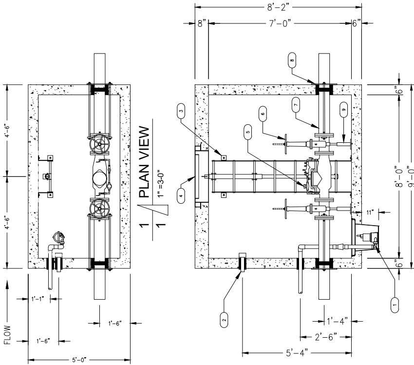
1 PLAN VIEW 1" = 3'-0"
