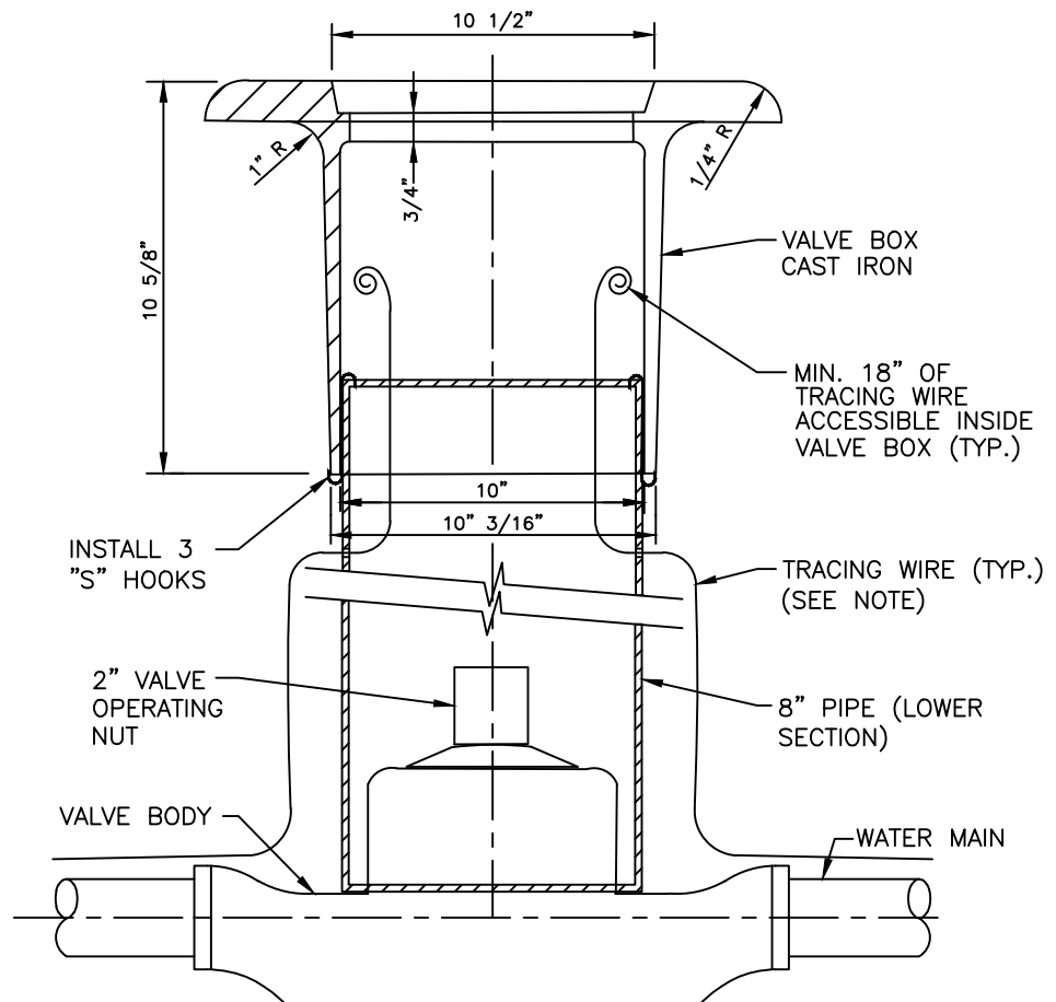
SECTION VALVE BOX
